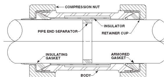
Style 90 Insulating Coupling Provides Seal Only and Insulating End
