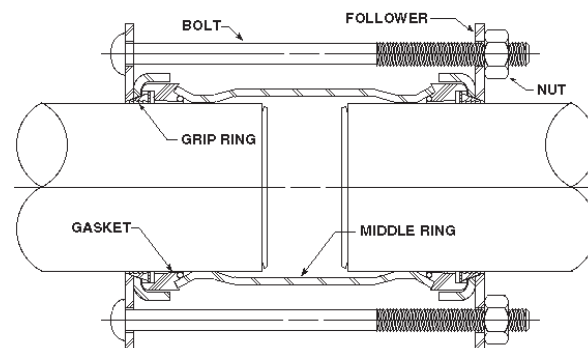
Style 711 Coupling
